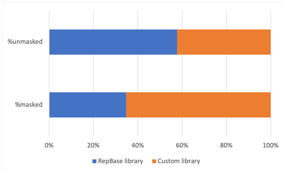
Figure 4: Number of bases repeat masked (blue) and unmasked (orange) per species using the "rebase_vertebrates" repeat library.
